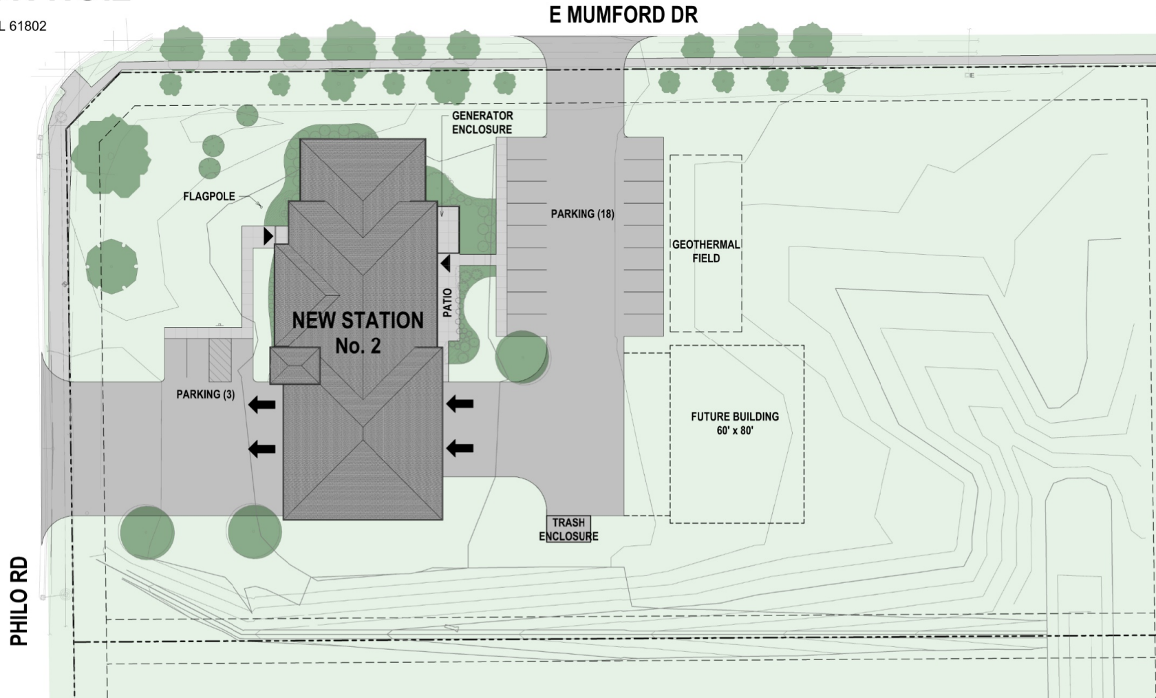
STATION 2 - SITE PLAN
